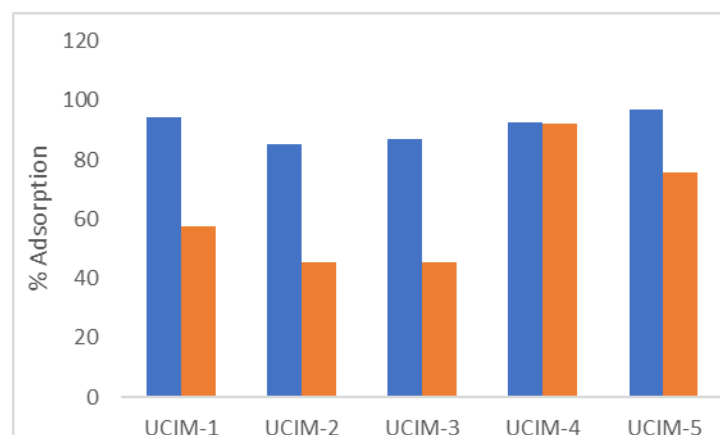
Fig. 4. Bar chart showing percentage adsorption of \text{Ca}^{2+} and \text{Fe}^{2+} by the different metal phosphonate nanoparticles (Source: Ogar, 2015)
