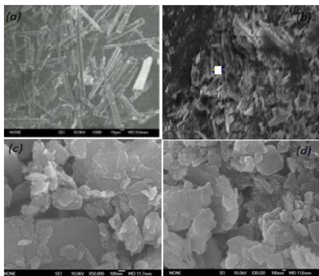
Fig. 3. Representative SEM micrographs (a) UCIM-1 (b) UCIM-2 (c) UCIM-3 (d) UCIM-4
