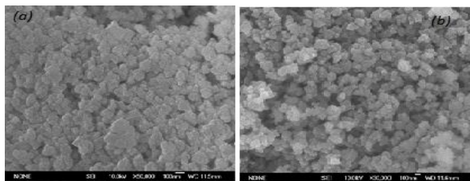
Fig. 5. SEM images of particles grown in (a) EMIMOAC (b) BMIMOAC
